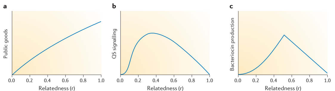
Figure 2 | Some relationships between genetic relatedness (r) and social behaviours. The production of public goods, such as siderophores, increases monotonically as relatedness between social partners increases 28 (a). Quorum sensing (QS) signalling (b) and bacteriocin production (c) are both predicted to show a dome-shaped function of relatedness, with signalling 91 and bacteriocin production 70 maximized at an intermediate relatedness.
